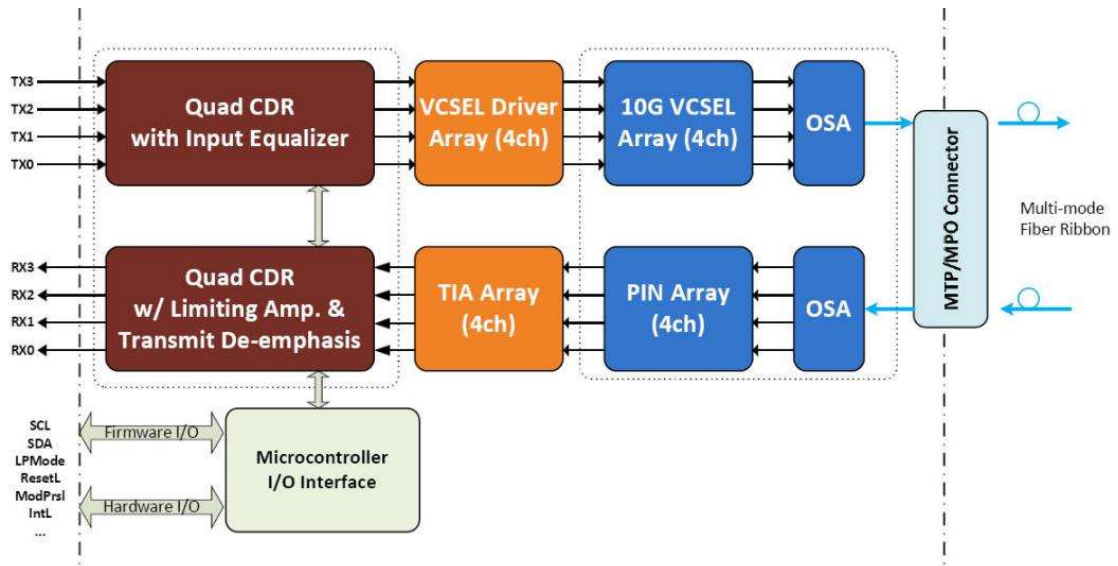
Figure1: Block Diagram
